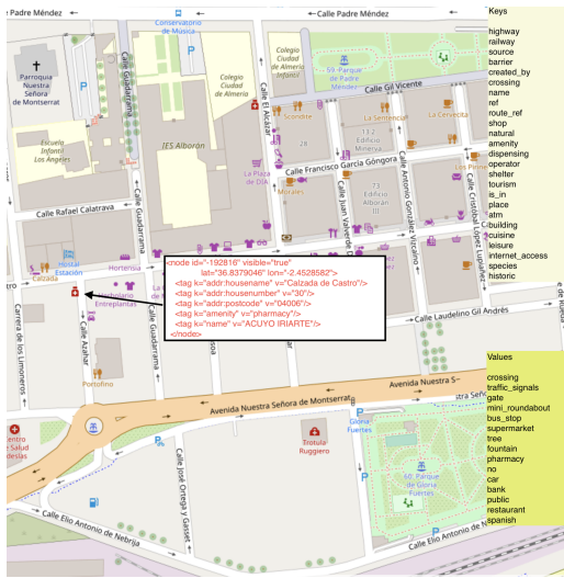
Figure 1. A graphical OSM of Almería (excerpt).
