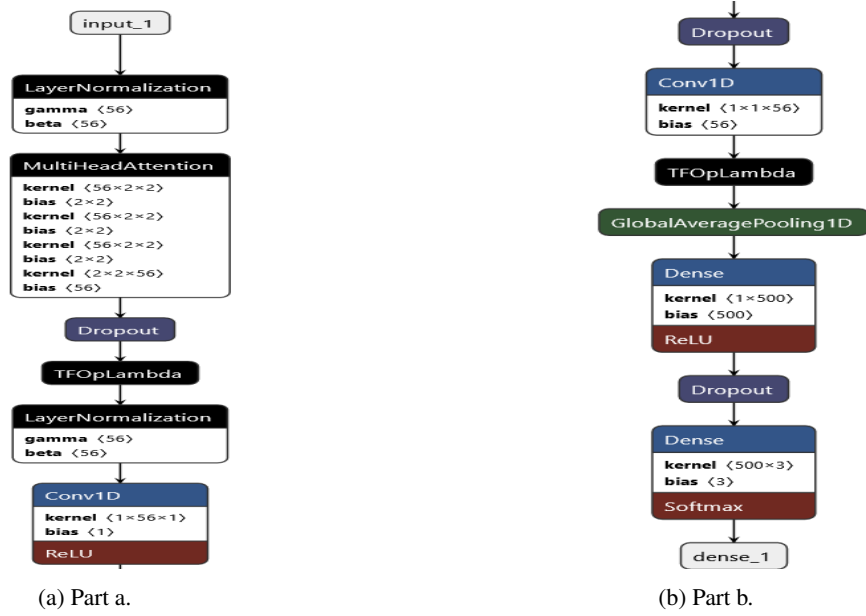
Fig. 2: Deep Transformer based Model structure
