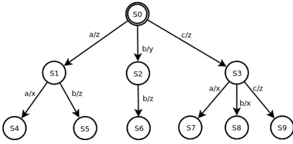
Figure 3: FSM example.
