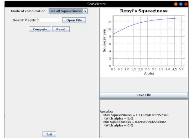
Figure 9: Squeeziness range mode example: Banckard case study.
