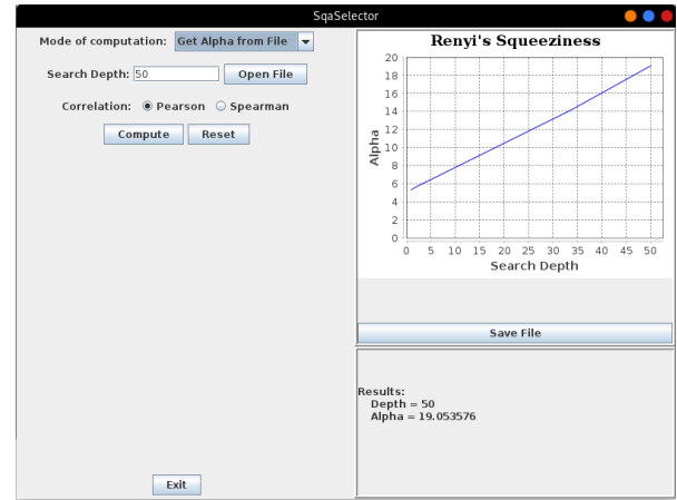
Figure 7: Alpha file mode example: TCP case study.
