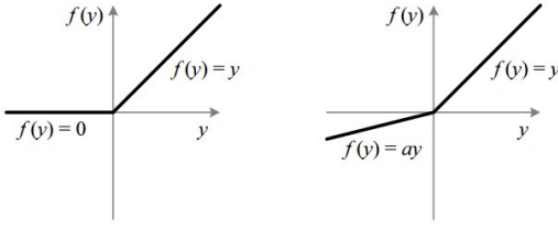
Figure 5: ReLU vs leaky ReLU.
