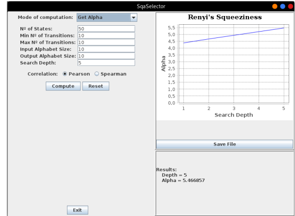
Figure 6: Alpha mode example: Coffee machine case study.
