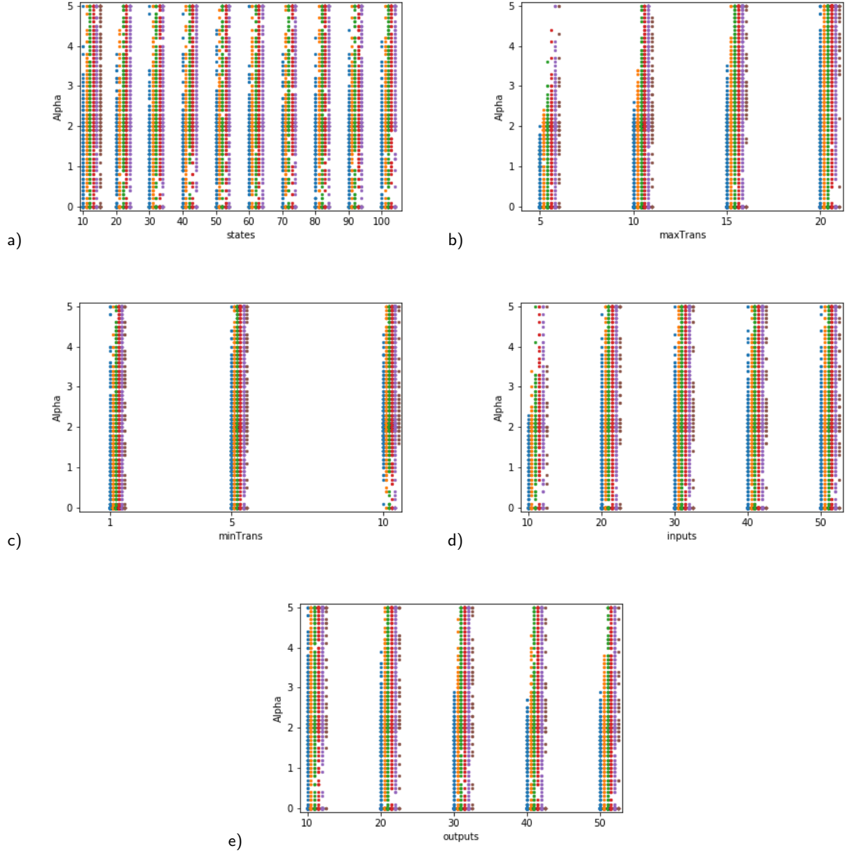
Figure 4: Correspondence between parameters and \alpha of elements of the dataset: states (a), maximum transitions (b), minimum transitions (c), input alphabet size (d) and output alphabet size (e).
