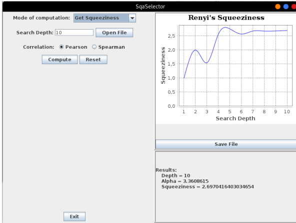
Figure 8: Squeeziness file mode example: Logic circuit case study.
