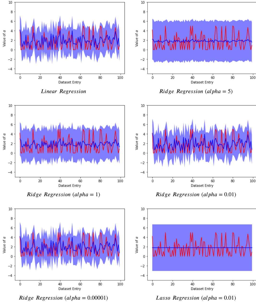
Figure 11: Confidence boundaries plots (part 1).
